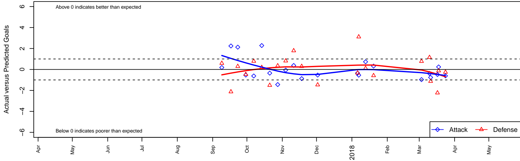
FWFC Select B04 Dots are actual minus expected GF (blue circles) and GA (red triangles). Blue line is smoothed change in attack strength. Red is smoothed change in defense strength.
